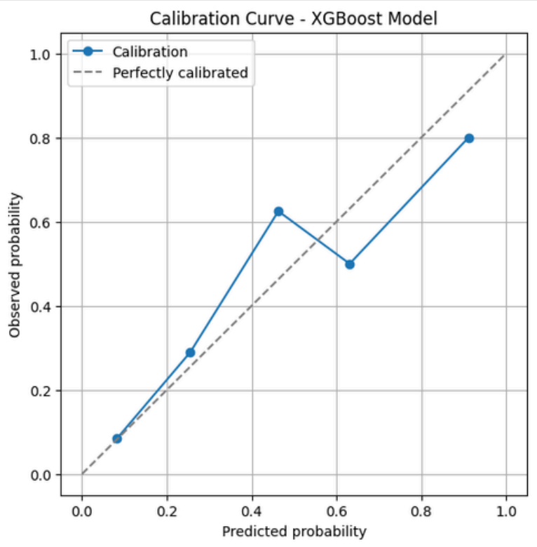
XGBOOST
